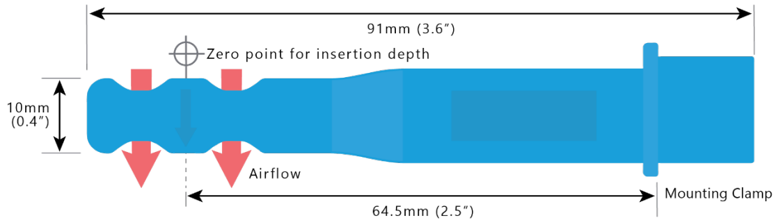
Mounting Figure 1: Sensor Dimensions
