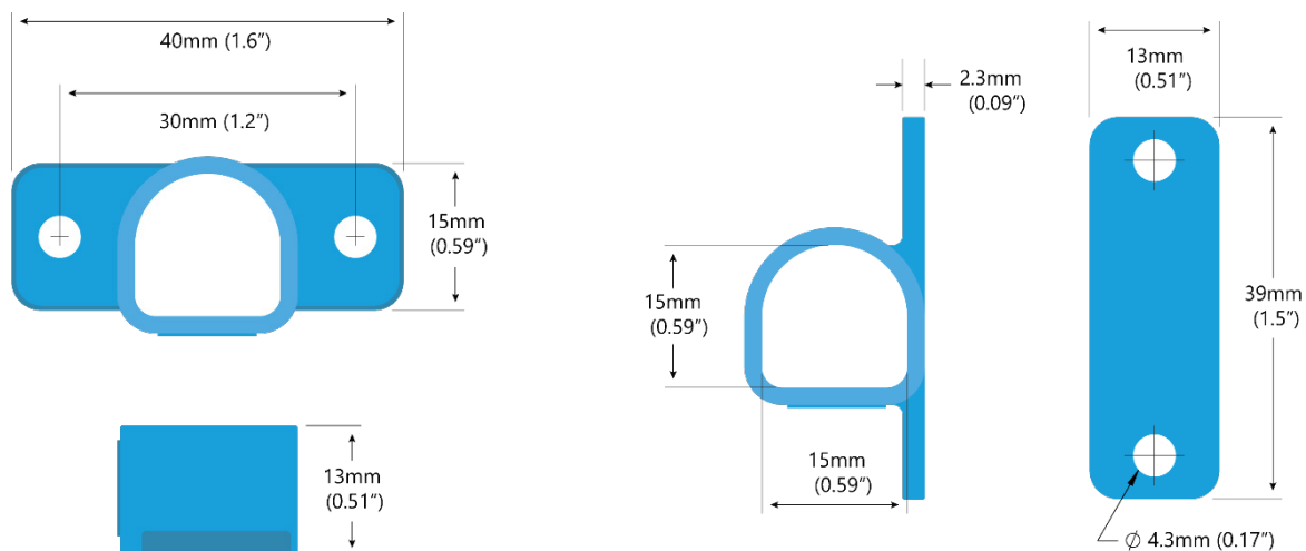
Mounting Figure 2: Brackets – Parallel (left) and Perpendicular (right)
